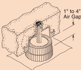
JACK-UP FLOOR Recommended Spacing 54"
